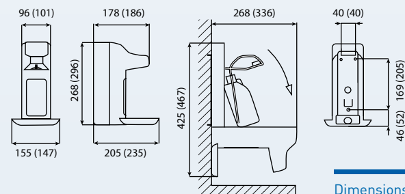
Dimensions in mm for the 500 ml dispenser (the values in brackets are valid for the 1.000 ml dispenser)
